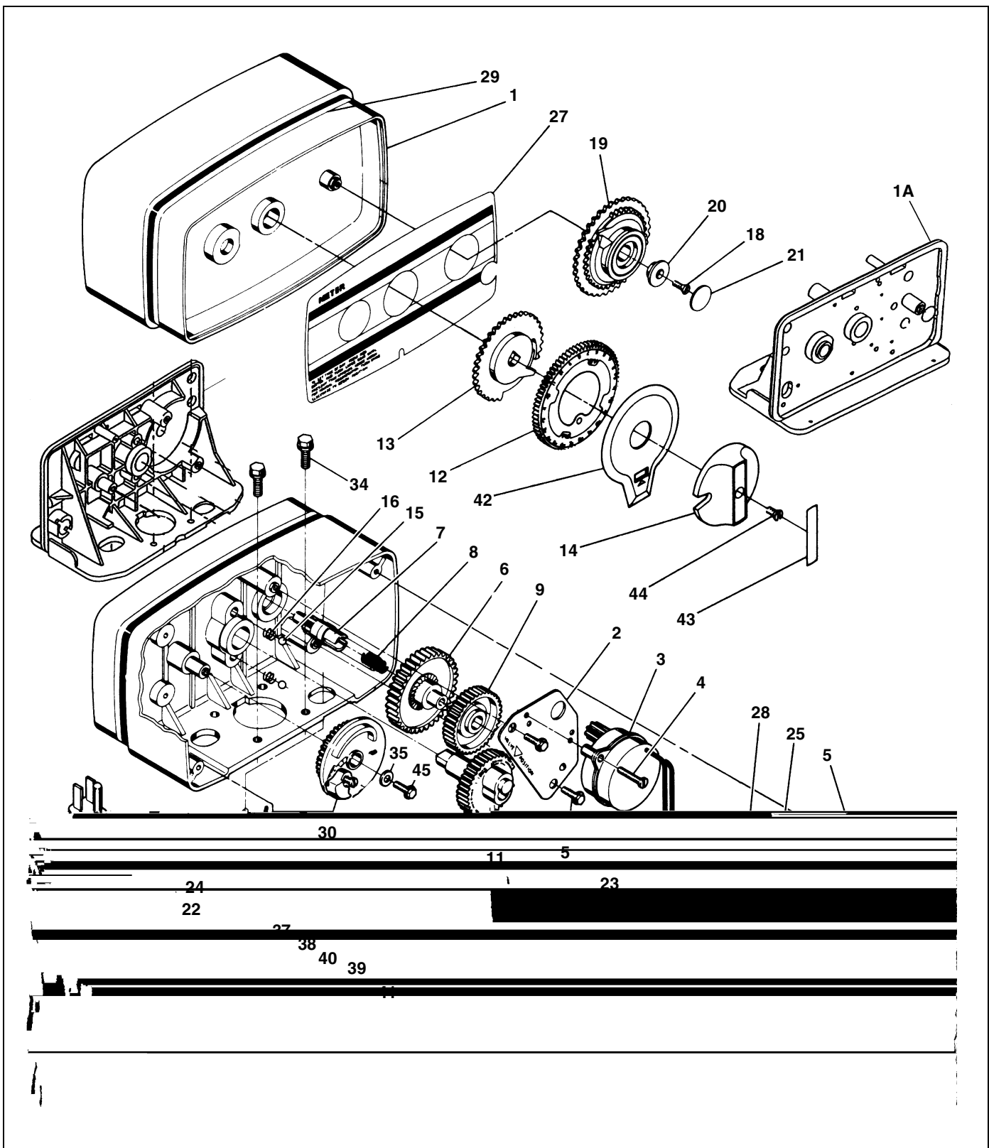
Figure 14: Model 5600 EDDF Control Valve Drive Assembly
